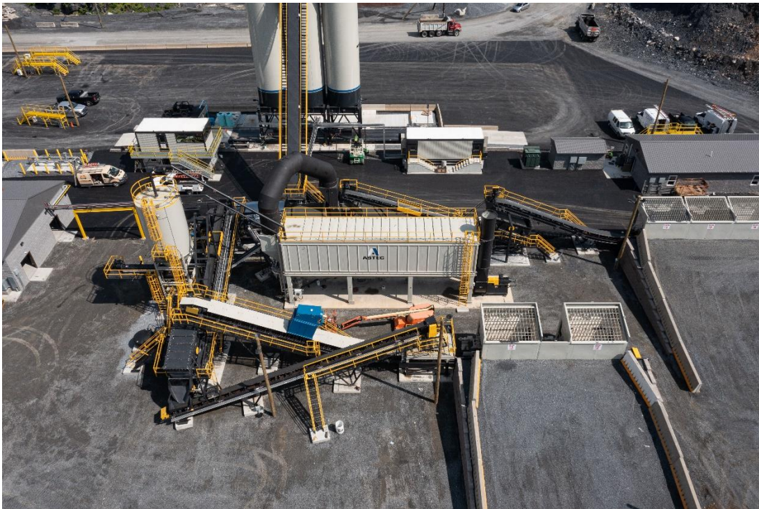
Precision fit and finish of the Easton Asphalt's new plant is evident in this pre-opening aerial drone photo from late June 2022.
